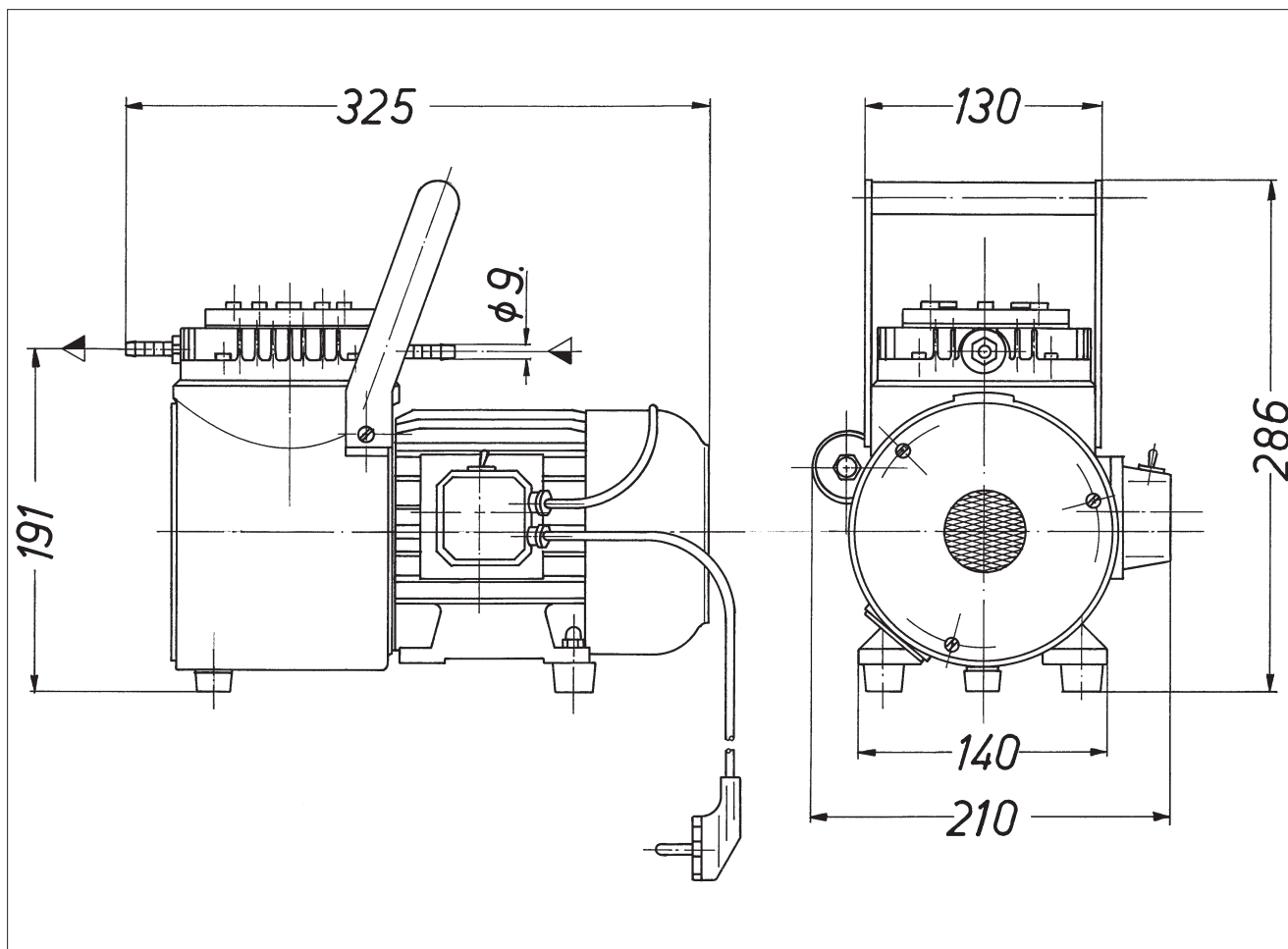
Dimensions (mm)
